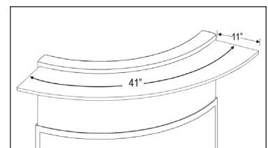
WKSRadius To be used with Quarter Round Inside Corner High Back 5526HB
